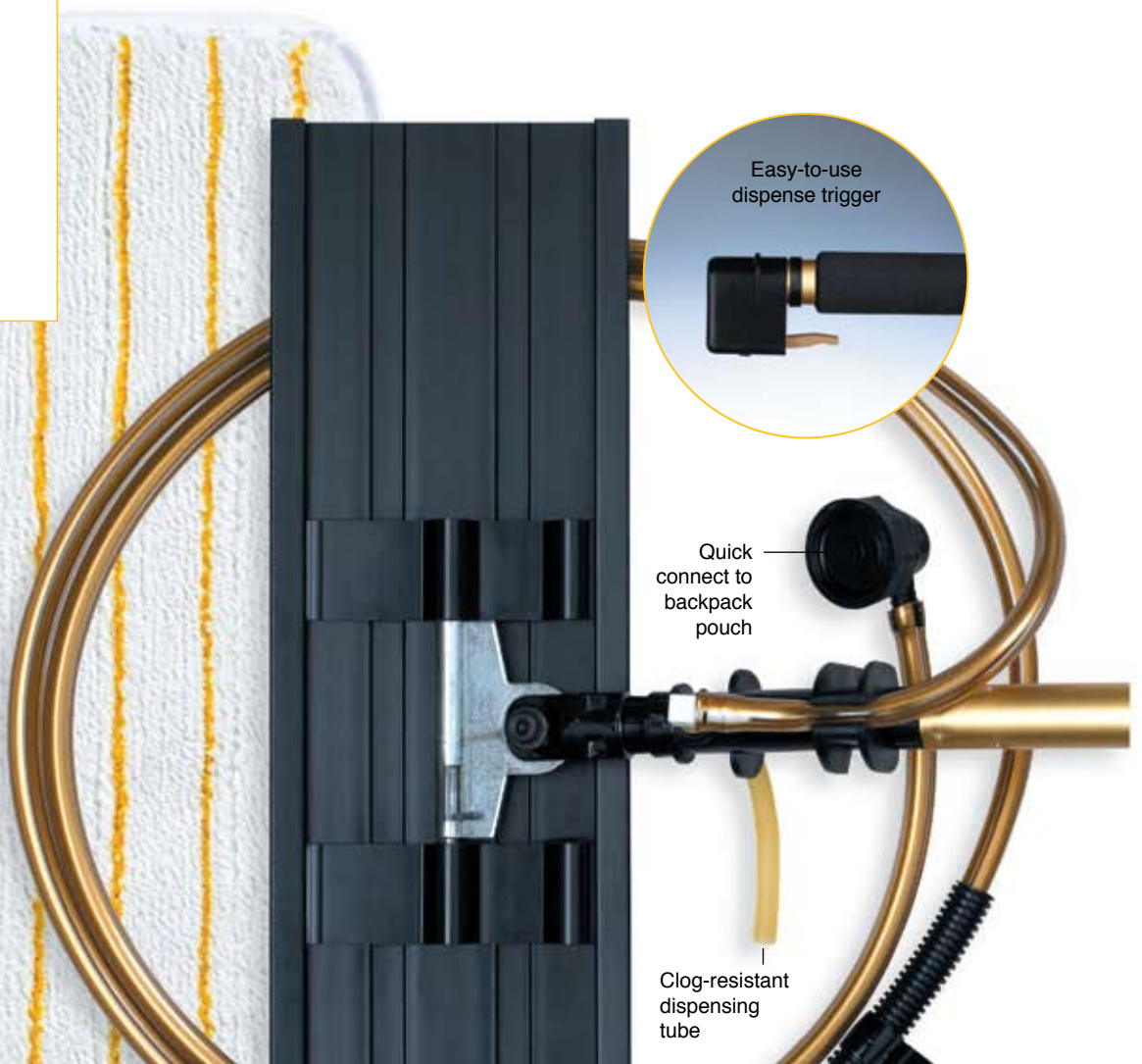
Refillable pouch
