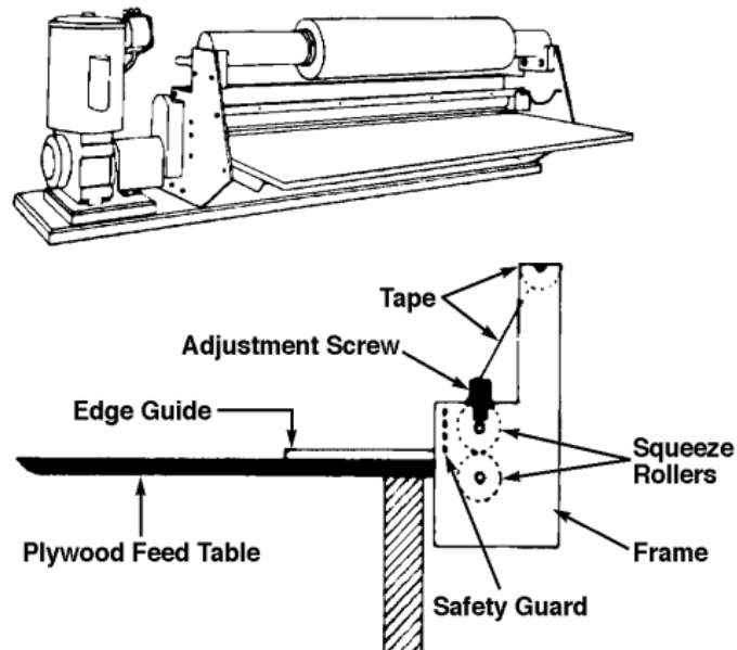
Figure 5. Examples of Mechanical Equipment
