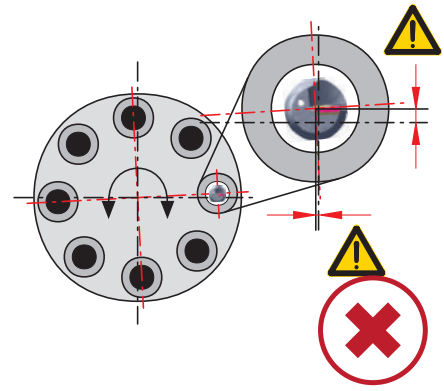
Turret position error
