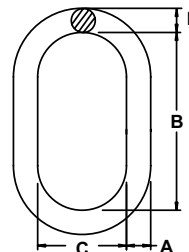
Can be used with included angles up to 120°
