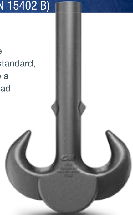
RAMSHORN FORM B HOOK (Drop Forged, Un-Machined)
