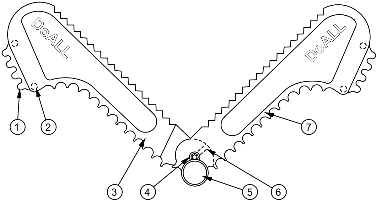
WORK HOLDER ASSEMBLY 040262
