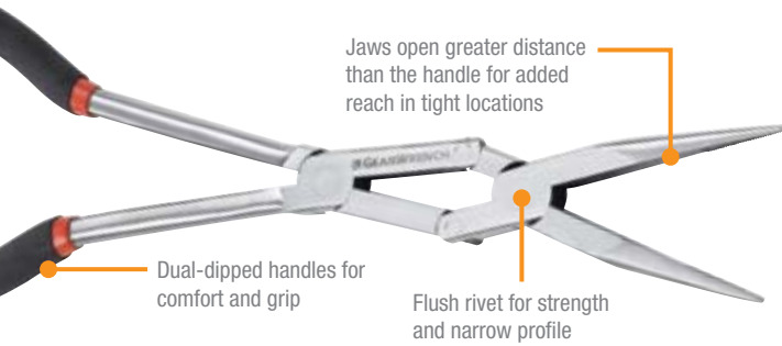
82005D Straight Double-X™ Pliers
