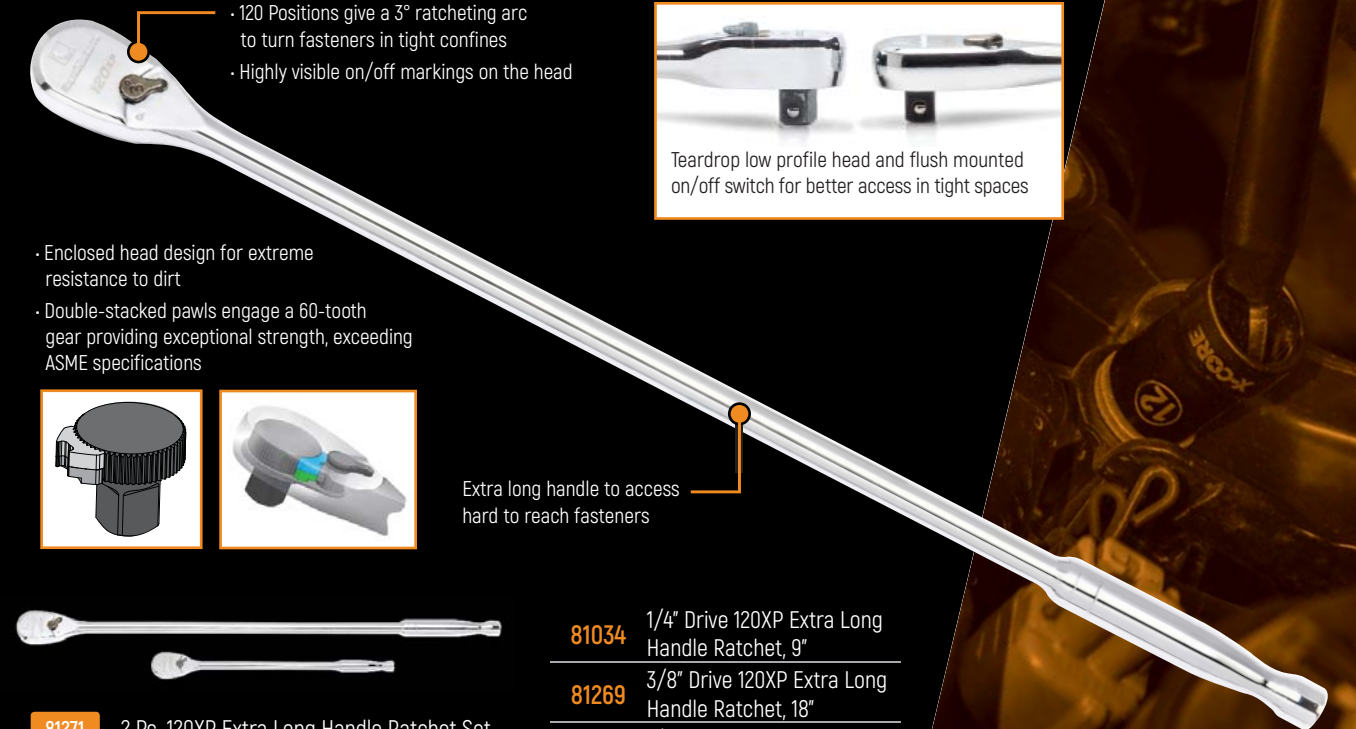
81364 1/2" Drive 120XP Extra Long Handle Ratchet, 24"
