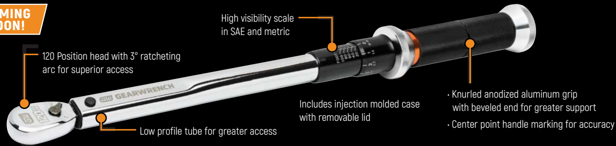
85171 1/4" Drive 120XP Micrometer Torque Wrench, 30-200 in. lbs.
