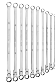
86126 10 Pc. 120XP™ Spline Metric XL GearBox Flex Ratcheting Wrench Set 10 - 19 mm
