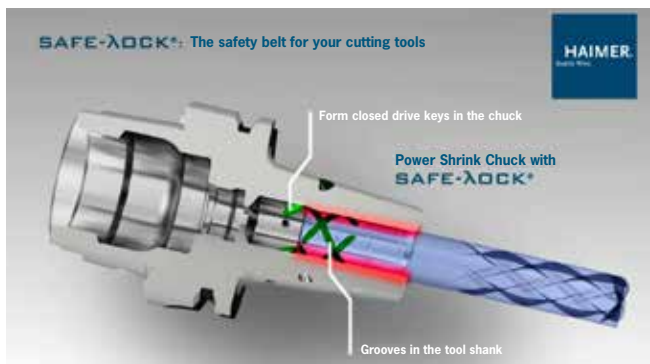
Power Shrink Chuck with SAFE-LOCK®
