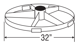
I-2030B Base
