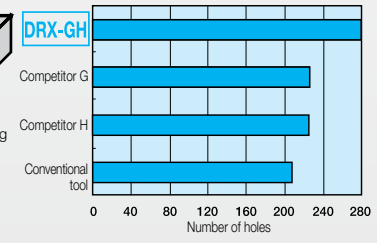
Interrupted drilling by displacing center of hole by 8mm
