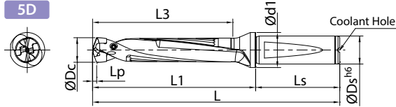
For Lp dimension, reference insert dimension table.
