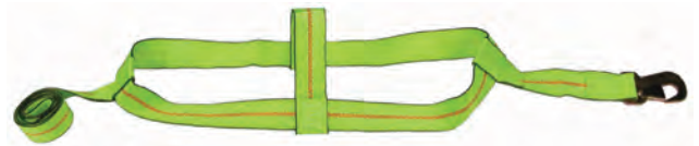
Snap Hook Basket Strap • 2" Web • Snap Hook WLL - 2,000 lbs. Used on Hydra-Tech® wheel lifts BSST
