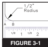
Figure 3-1. Measure the edge radius. The radius is equal to the distance between points A and B.
