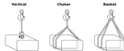
Figure 4-1. Common types of sling hitches
