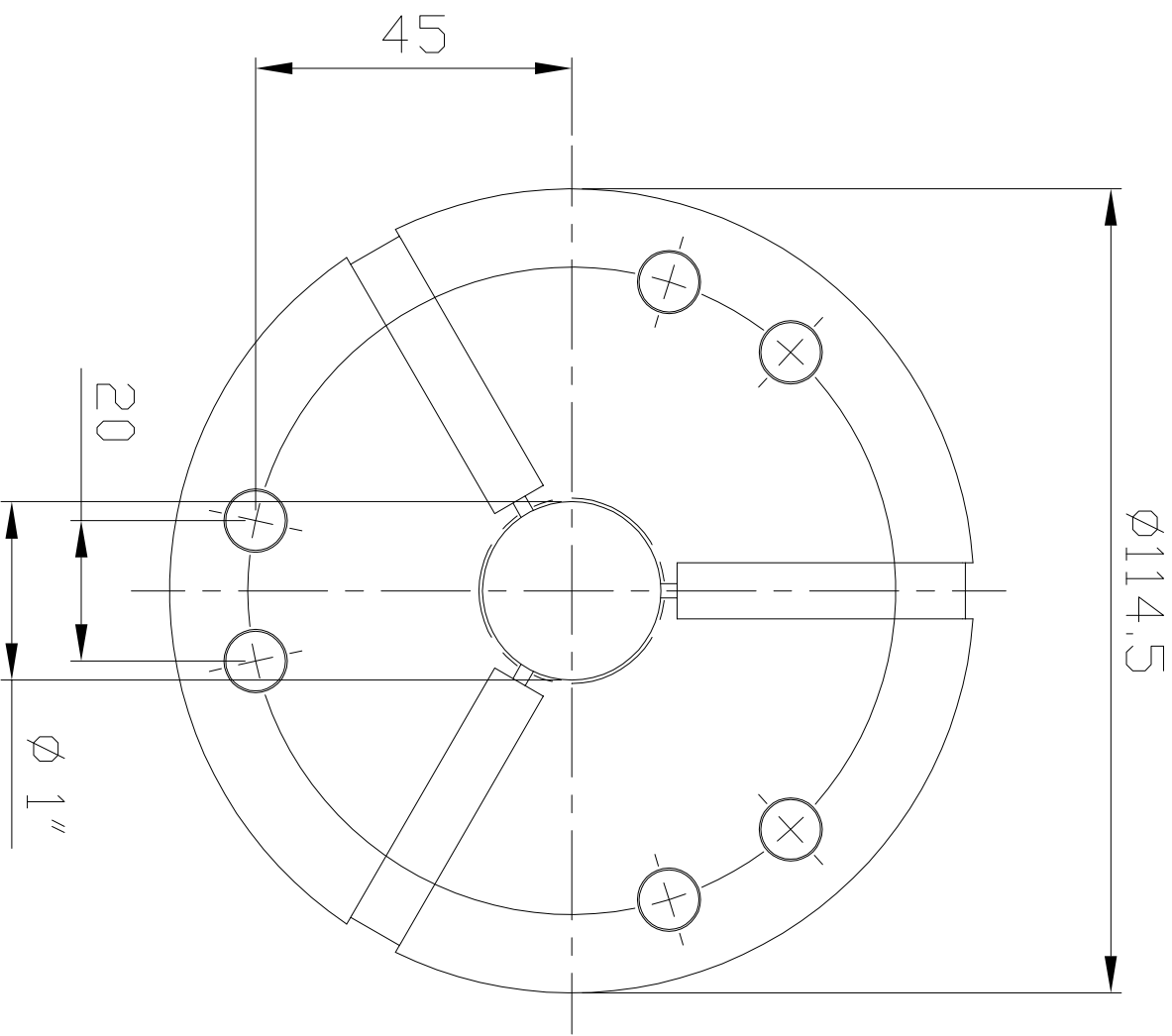
Serrated hole
