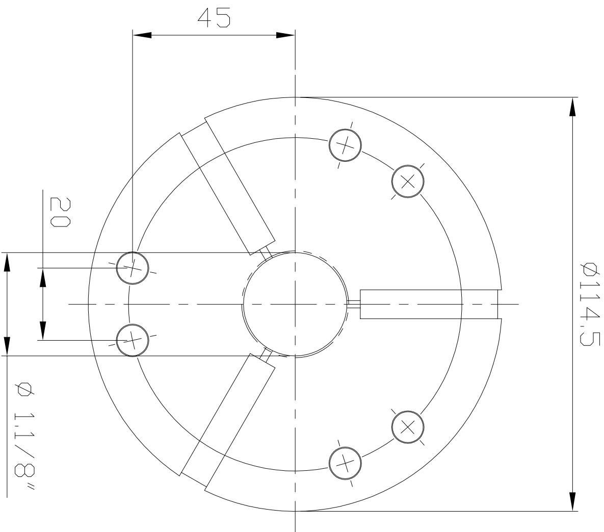
Serrated hole
