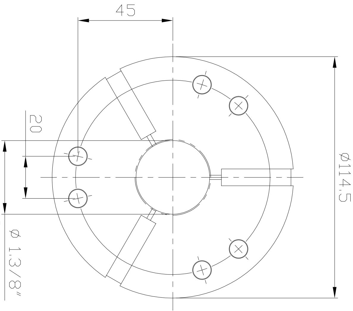
Serrated hole
