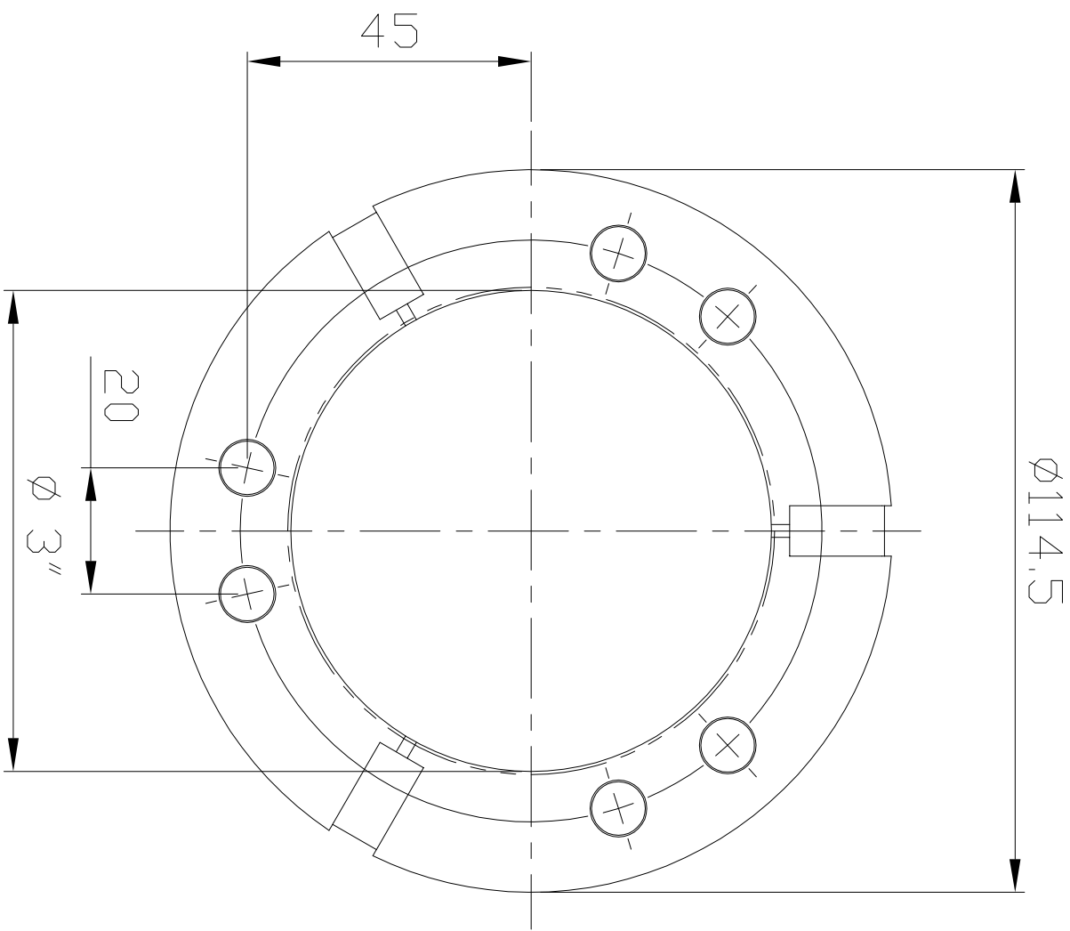
Serrated hole
