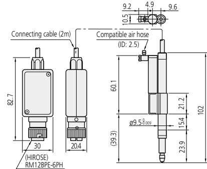
542-223: Air-lifter model
