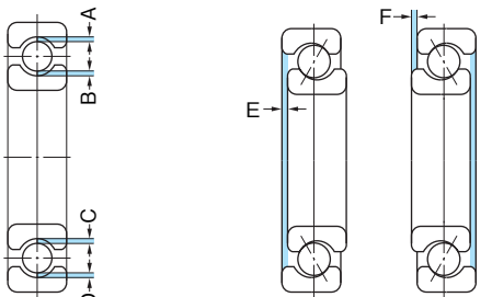
Fig 6.1 Radial internal clearance = A+B+C+D Fig 6.2 Axial internal clearance =E+F
