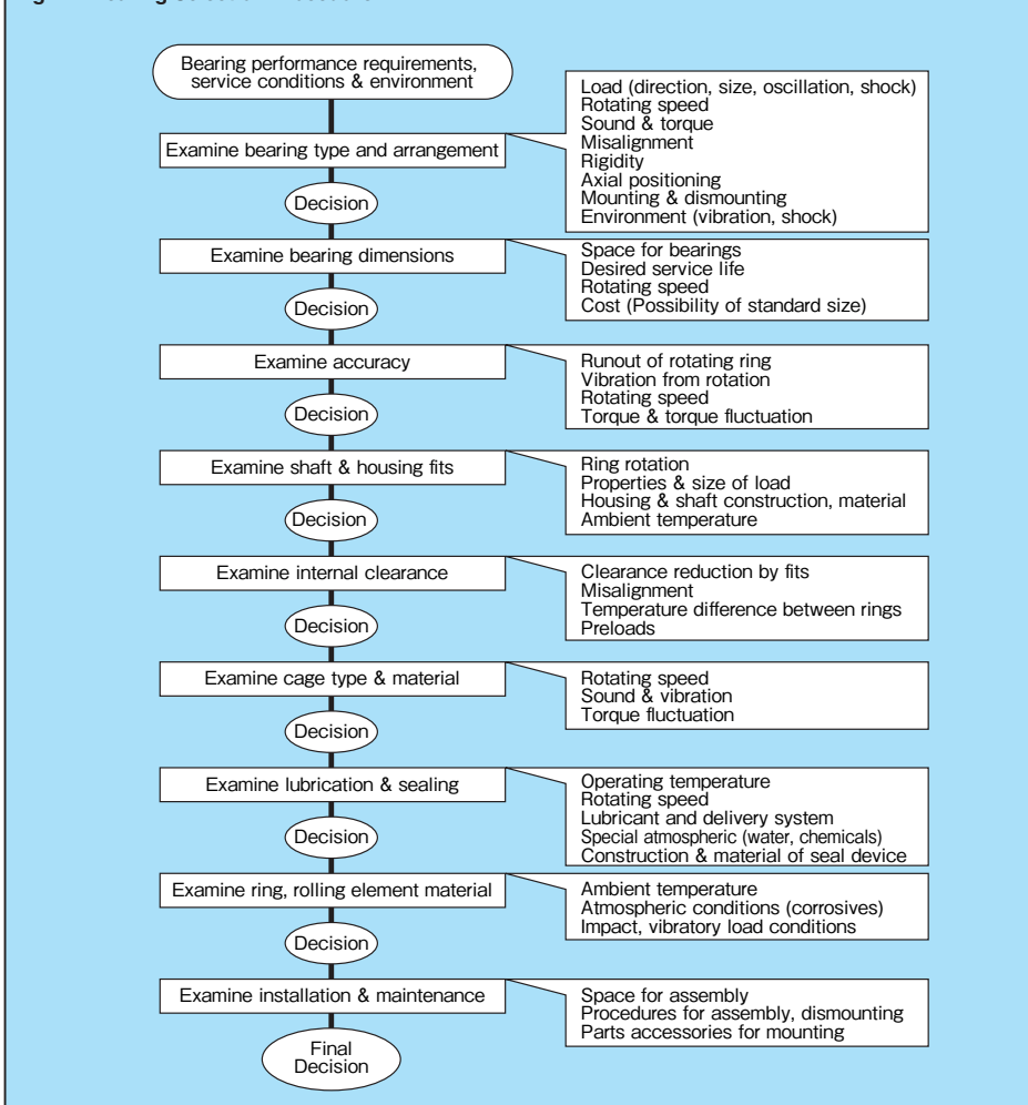
Fig. 2.1 Bearing Selection Procedure
