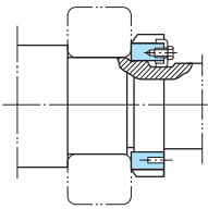
(b) Shaft Nut and Lock Plate
