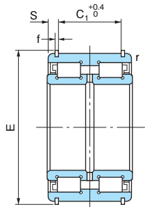
Shield type (E50...NR) with snap rings
