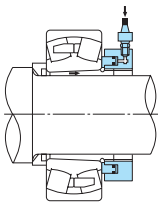
Fig 8.45 Hydraulic Nut
