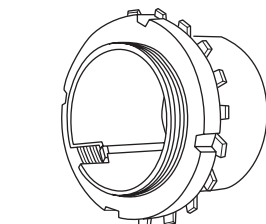
Fig. 8.15 Adapter Using Washer (Bearing Bore Diameter Number \leq 40 )
