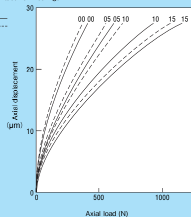
Fig. 8.4 Axial Load and Axial Displacement
