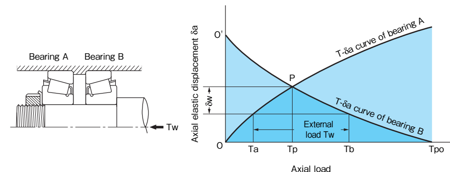
Fig. 8.5 Description of Fixed Position Preloading
