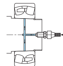
Dismounting Bearing with Oil Injector
