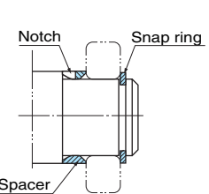
(b) Snap Ring and Notched Spacer
