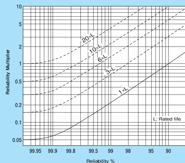
Fig 3.6 Reliability Graph
