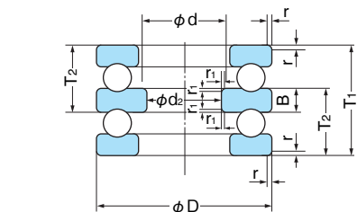
Fig 4.4 Double-direction Thrust Ball Bearings
