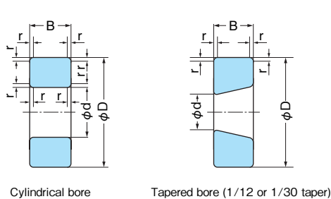
Fig 4.1 Radial Bearings (except Tapered Roller Bearings)
