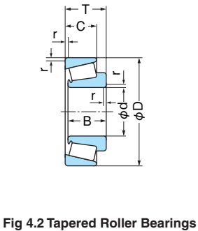
Fig 4.2 Tapered Roller Bearings
