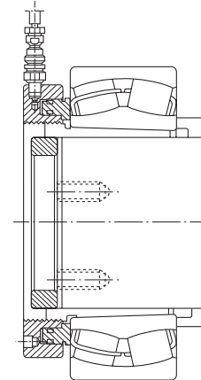
Fig.4. Sleeve thread
