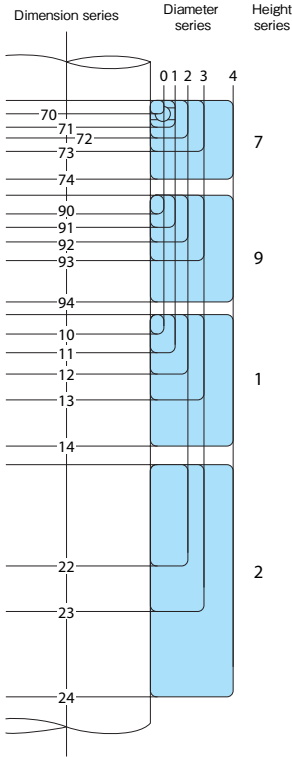
Fig 4.7 Graphical Representation of the Dimension series of Thrust Bearings (except diameter 5 series)
