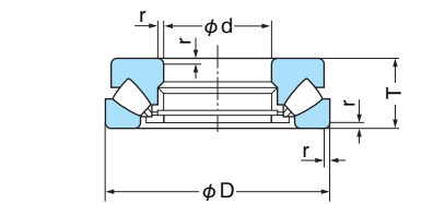
Fig 4.5 Spherical Roller Thrust Bearings
