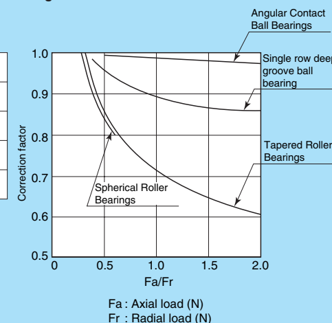
Fig. 8.38.2 Correction Factor for F_a/F_r
