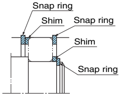
(c) Snap Ring and Spacer
