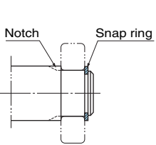
(a) Snap Ring and Notched Shoulder
