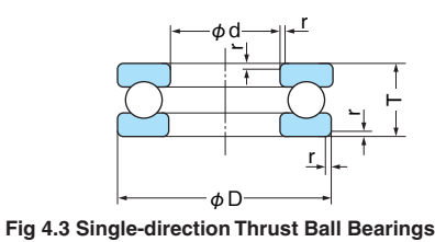
Fig 4.3 Single-direction Thrust Ball Bearings
