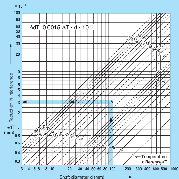
Fig. 8.2 Reduction in Interference of Inner Ring Due to Temperature Difference
