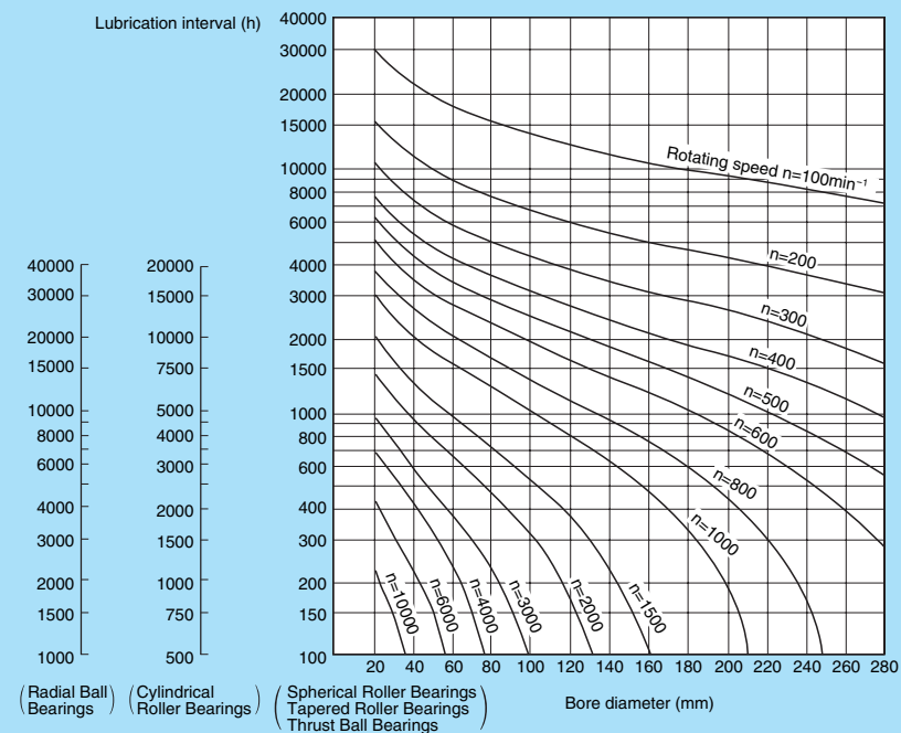
Fig 8.37 Grease lubrication interval
