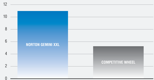
Norton Gemini XXL 9" x 1/4" Wheels – Grinding Ratio (Cut Rate/Life)
