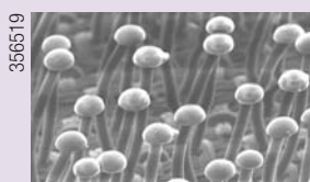
Hook Type 4 Hook-and-Loop Tall Mushroom Hook (250HD)
