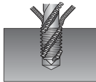
R40/R45 Blind holes ULDR = 2,5
