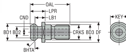
Design 3 = With through coolant
