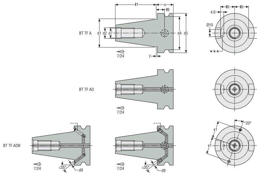
BT30 TF and 50 ADB with sealing dowel
