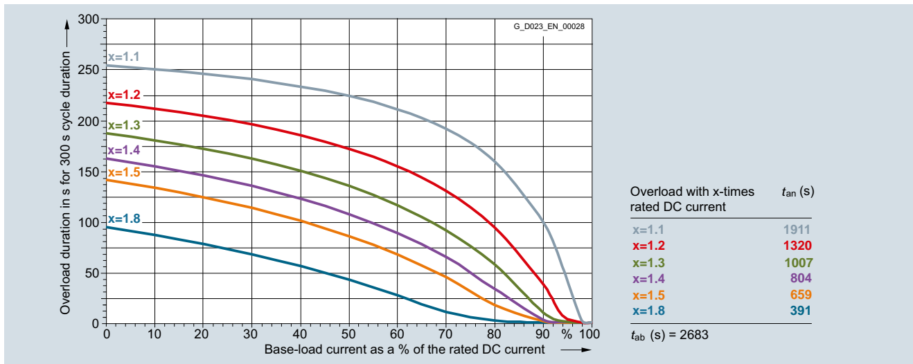
6RA8028-6DV62-0AA0 90 A/four-quadrant operation 400 V, 6RA8028-6FV62-0AA0 90 A/four-quadrant operation 480 V
