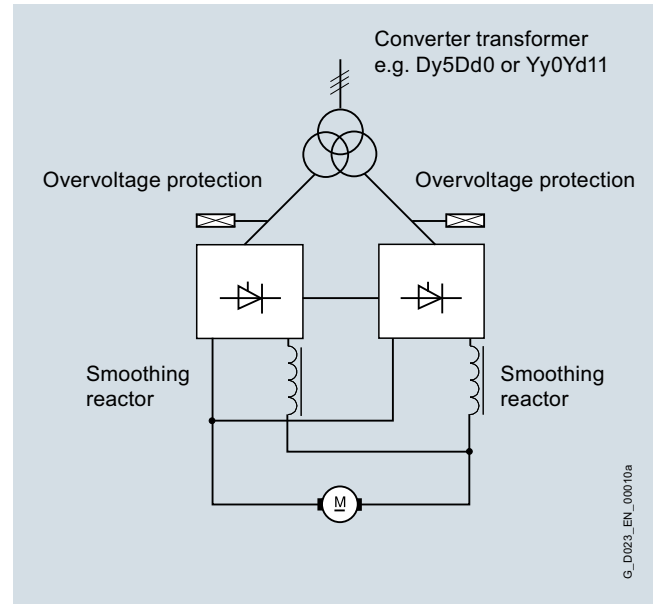
12-pulse operation
