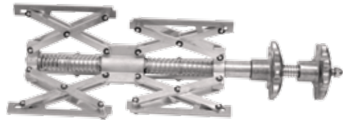
4" - 8" (100-200 mm) Internal Fit-Up Clamp
